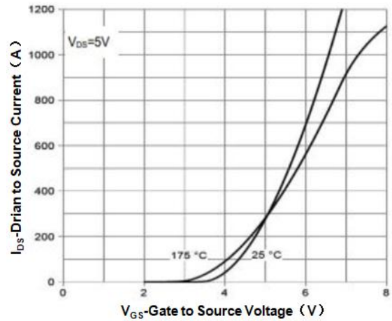
Transfer Characterisics
