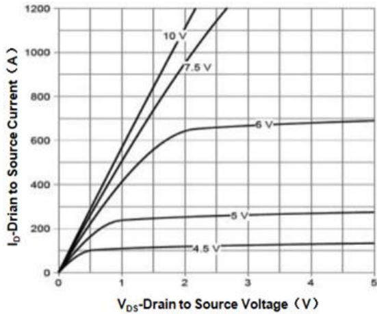
Output Characterisics
