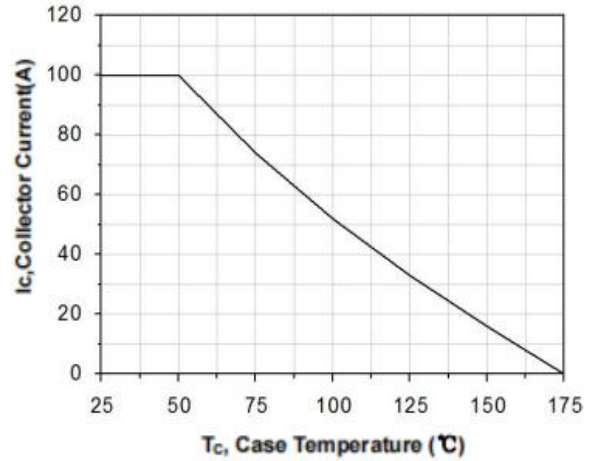
Collector current as a function of case temperature ( V_{GE} \geq 15\text{V} , T_j \leq 175^\circ\text{C} )
