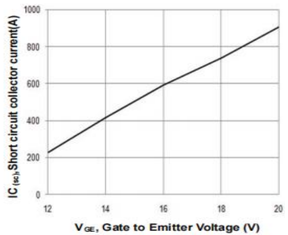
Typ. short circuit collector current as a function of gate-emitter voltage (VCE ≤ 400V, Tj ≤ 150°C)
