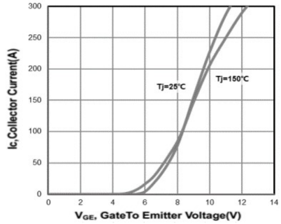
Transfer Characterisics
