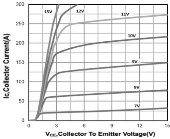
Output Characterisics
