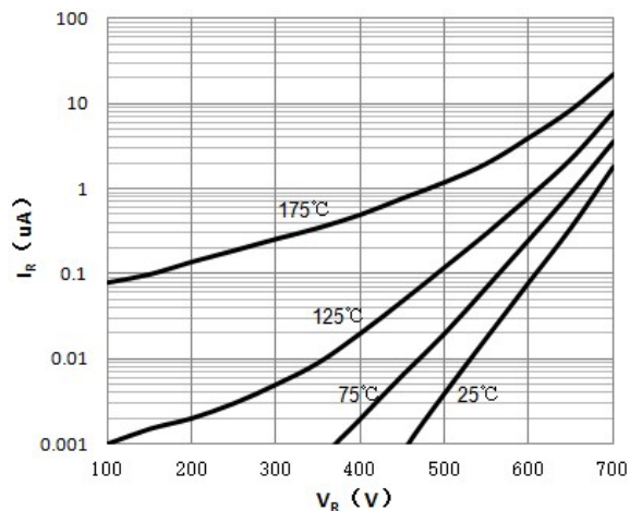
Reverse Characteristics
