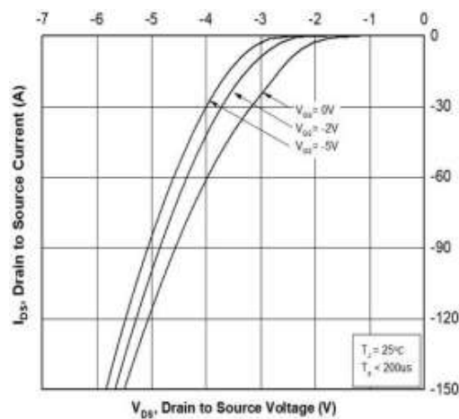
Source-Drain Diode Characteristics
