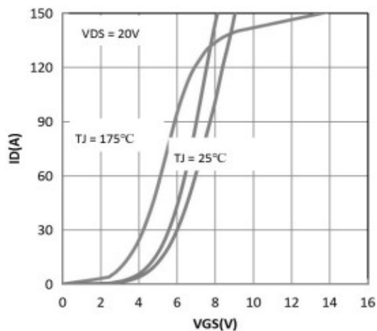
Transfer Characteritsics
