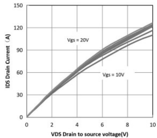
Output Characteritsics T J =175°C
