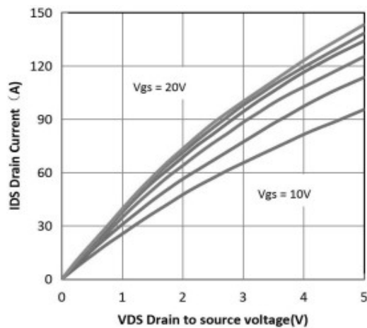
Output Characteritsics T J =25°C
