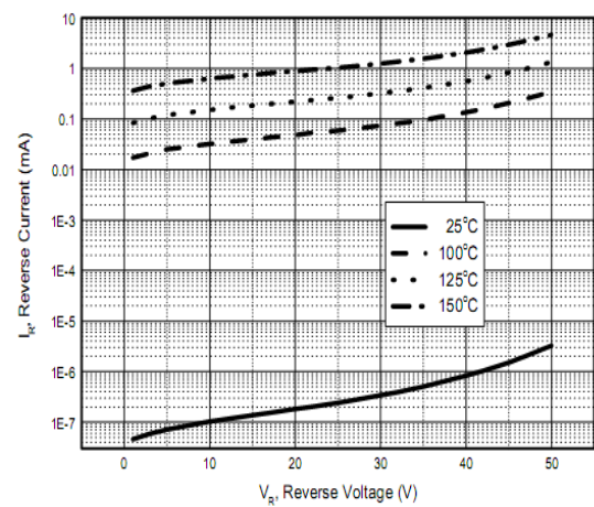
Reverse Characteristics Per Diode
