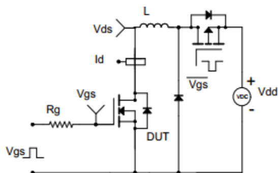
Unclamped Inductive Switching (UIS) Test Circuit & Waveform
