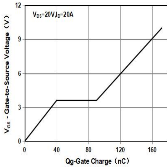
Gate Charge Waveform
