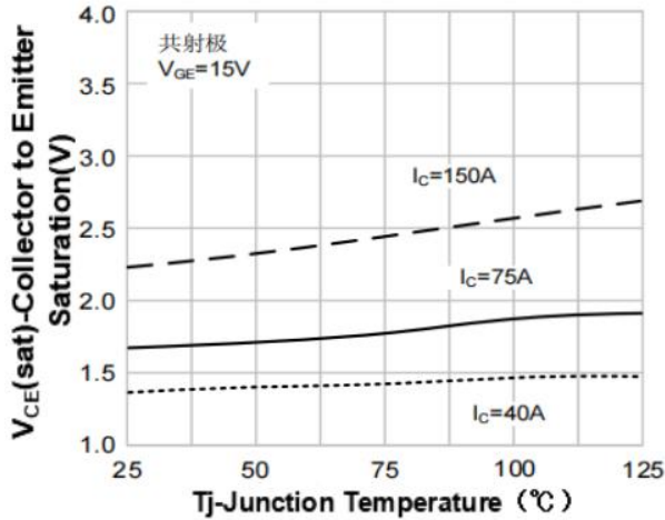
Typical collector-emitter saturation voltage as a function of junction temperature ( V_{GE} = 15V )
