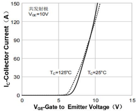
Transfer Characteristics( V_{GE}=20V )
