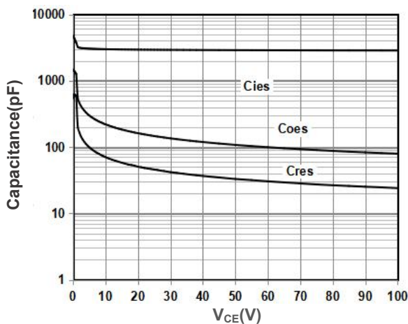
Capacitance
