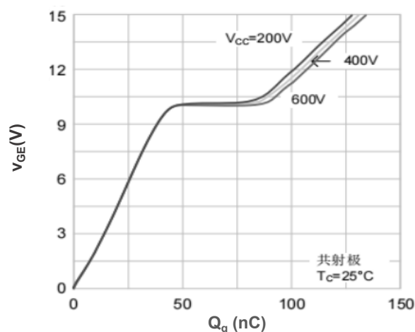
Typical gate charge
