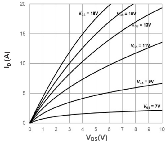
Output Characteritsics T_J = 175^\circ\text{C}
