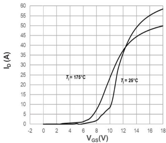
Transfer Characteritsics
