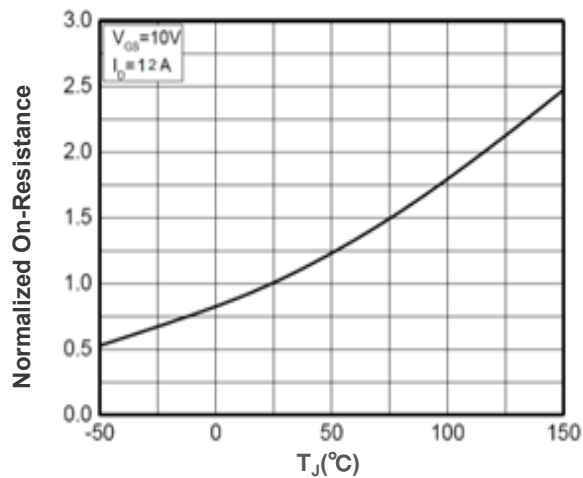
Rdson-Junction Temperature
