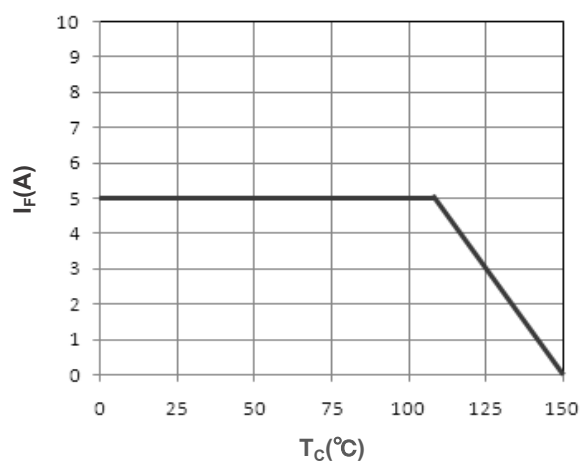
Current Derating Per Diode
